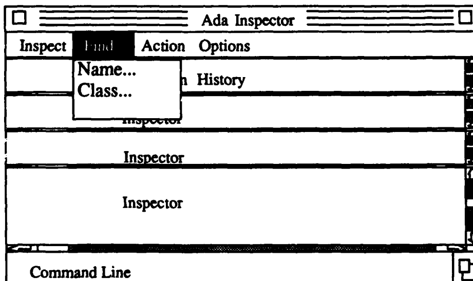
Figure 8-9. Find Menu
